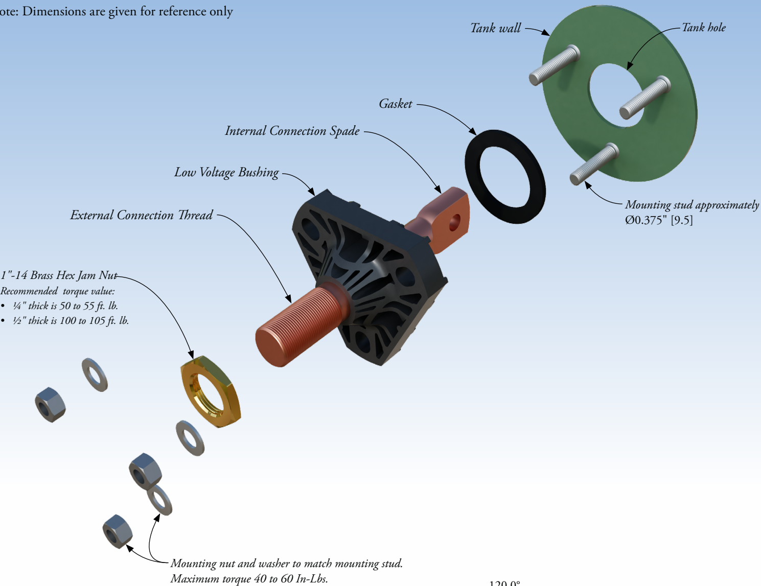
Figure 1 Mounting
